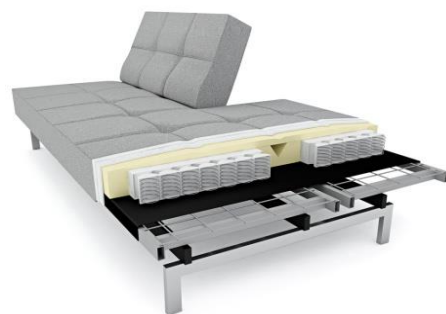
Cross-section-view
