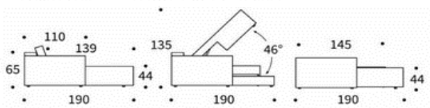
Headrest FLIP adjustable in height & angle
